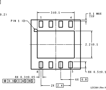
8-Lead LLP Order Number LM2940LD-5.0, LM2940LD-8.0, LM2940LD-9.0, LM2940LD-10, LM2940LD-12 or LM2940LD-15 NS Package Number LDC08A
