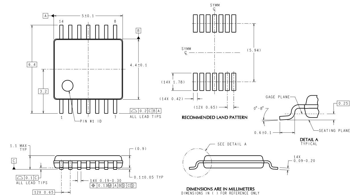
14-Pin TSSOP NS Package Number MTC14
