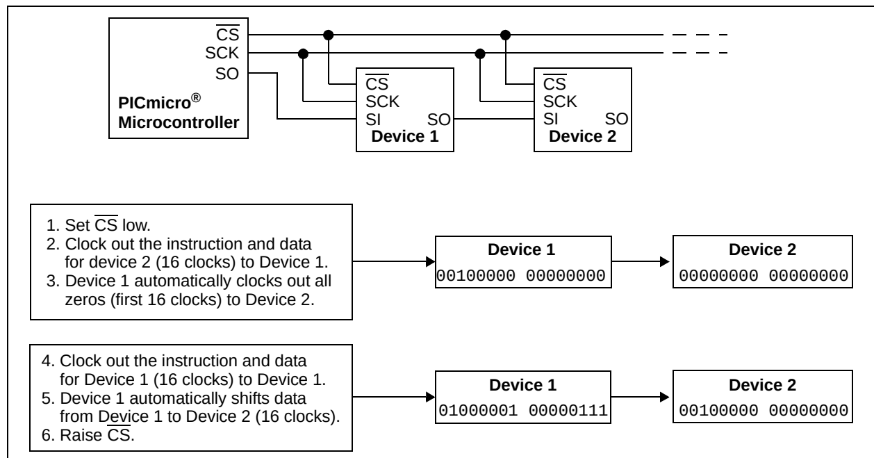
FIGURE 5-3: Daisy-Chain Configuration.
